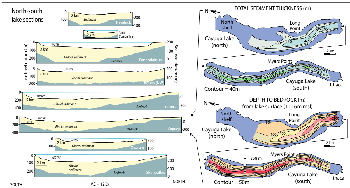
Figure 12. Section and map views of sediment fill statistics of the Finger Lakes, New York State (after Mullins et al., 1995) A) Total thickness of the glacial sediment fill in the various Finger Lakes. B) Total thickness isopach of glacial sediment fill (m) and depth to bedrock isoclinal relative to lake water surface (based on Mullins et al., 1996 seismic interpretation, this has been refined by current interpretation detailed earlier in this report).
