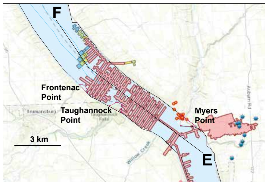
Figure 3. Location of cross sections, downcutting of Onondaga Formation and present mine location (red) and future mining areas (blue). Base map from Karen 2017. The deepened valley floor resulting in thin overburden over Syracuse Formation is expected to be inside the blue area.
