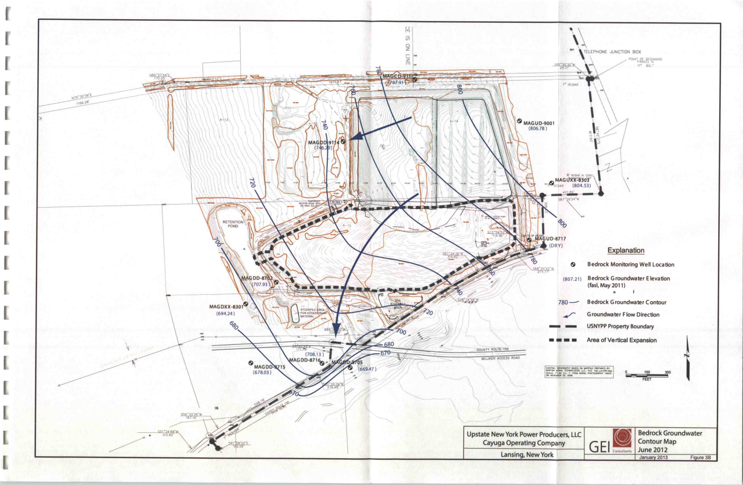
Figure 2 Potentiometric Surface Diagram June 2012 Bedrock Aquifer
